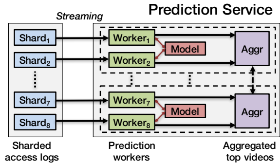
Figure 3: CHES video prediction service architecture.
